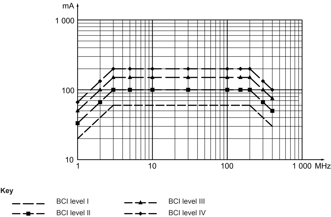
Figure E.1 — Test severity levels and frequency bands (BCI)
